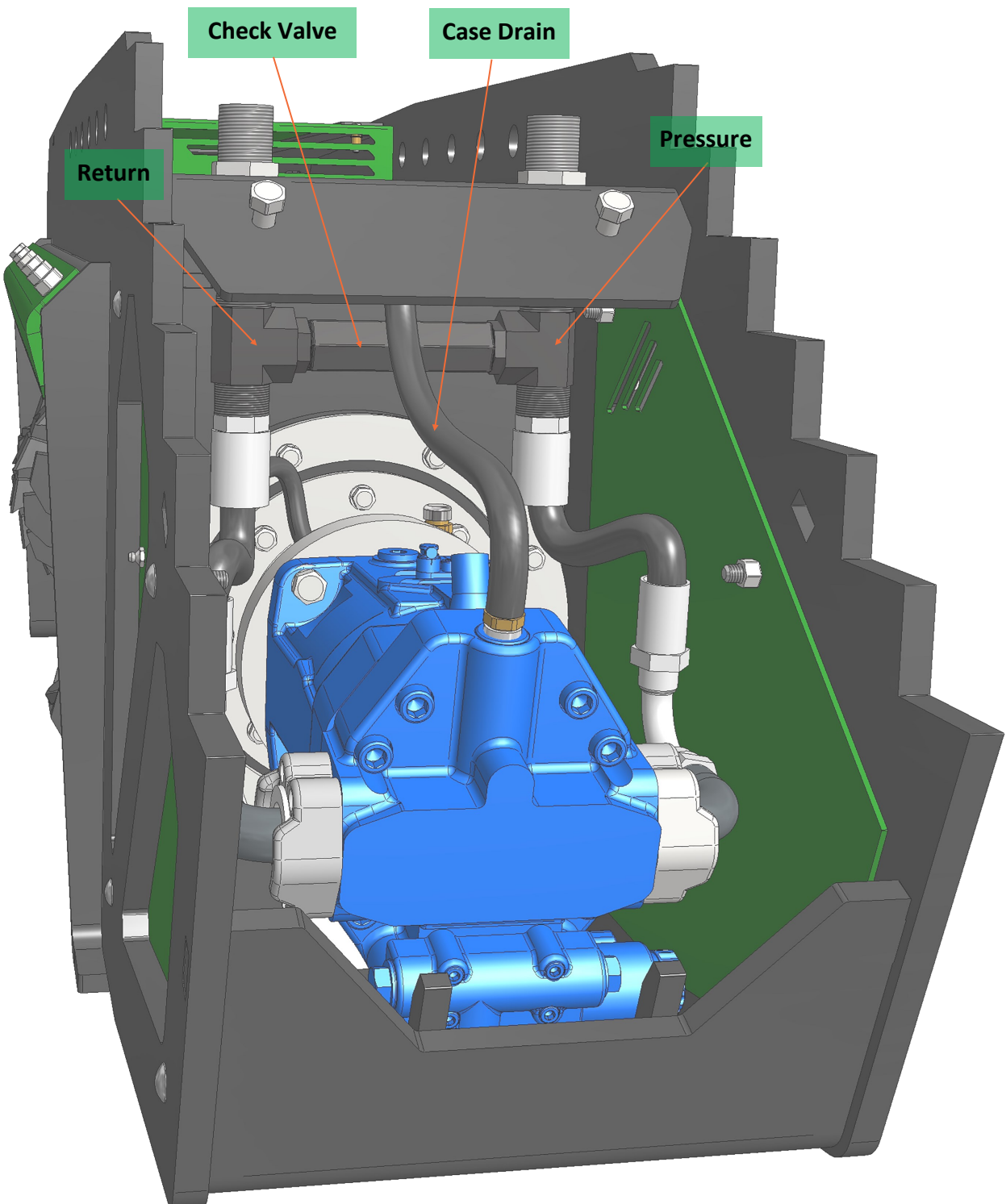
Hydraulic plumbing
